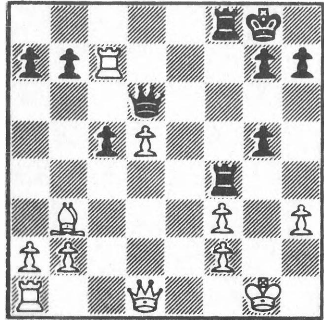
158 After 18...Raf8
